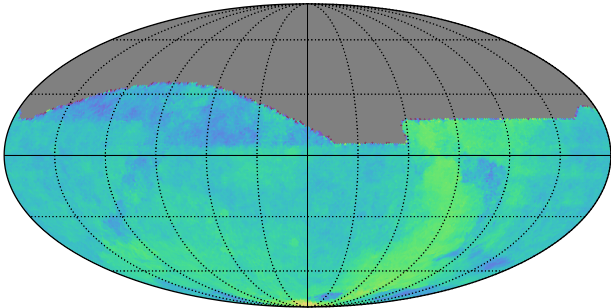
ddf_loaded_half_fl1_v3.4_10yrs All sky: Parallax Coverage @ 24.0
