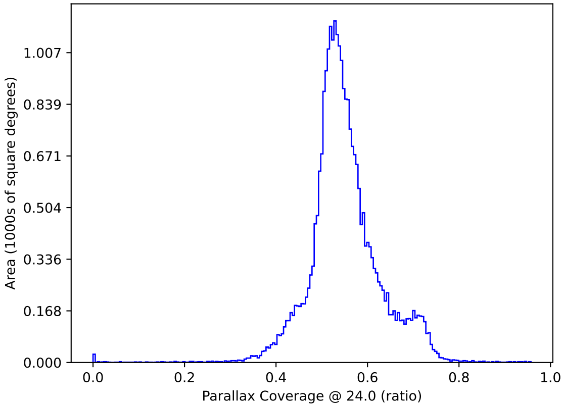
ddf_loaded_half_fl1_v3.4_10yrs All sky: Parallax Coverage @ 24.0
