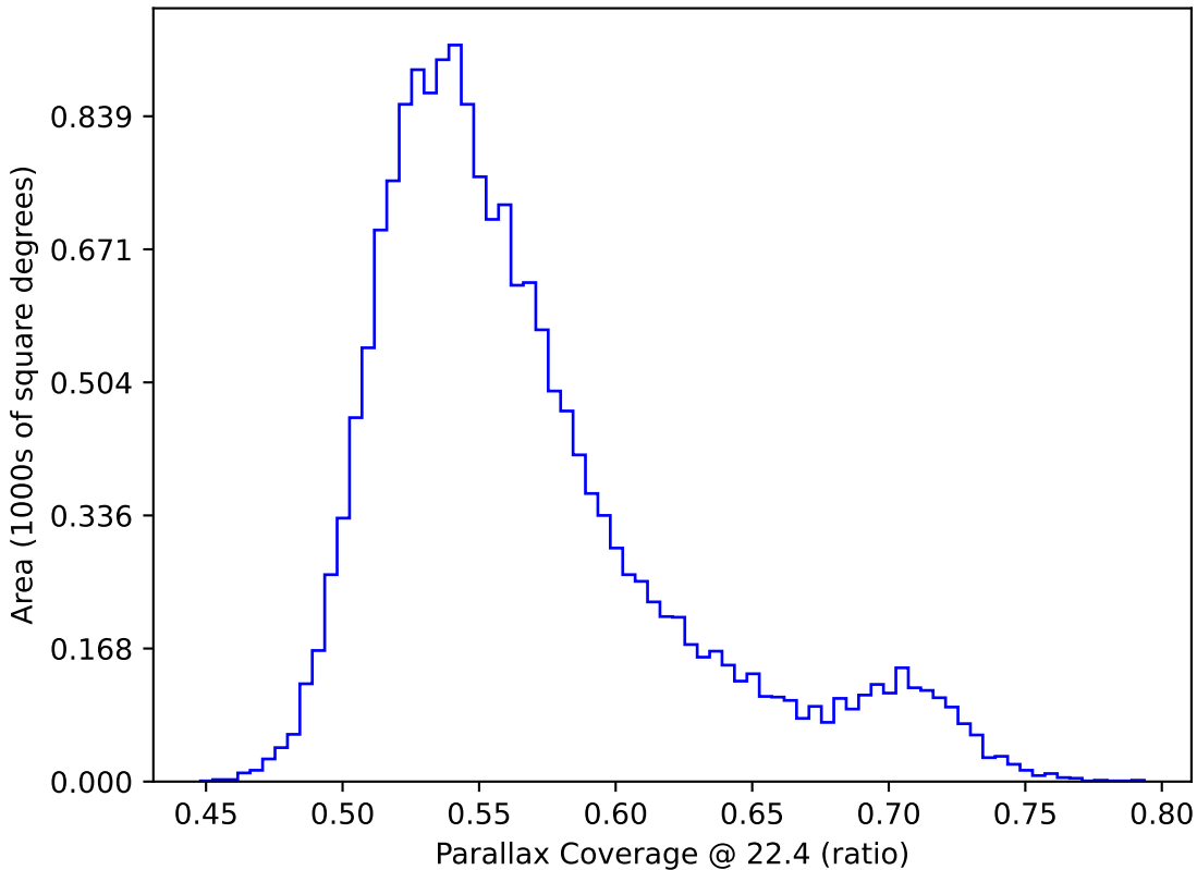
ddf_loaded_half_fl1_v3.4_10yrs WFD: Parallax Coverage @ 22.4
