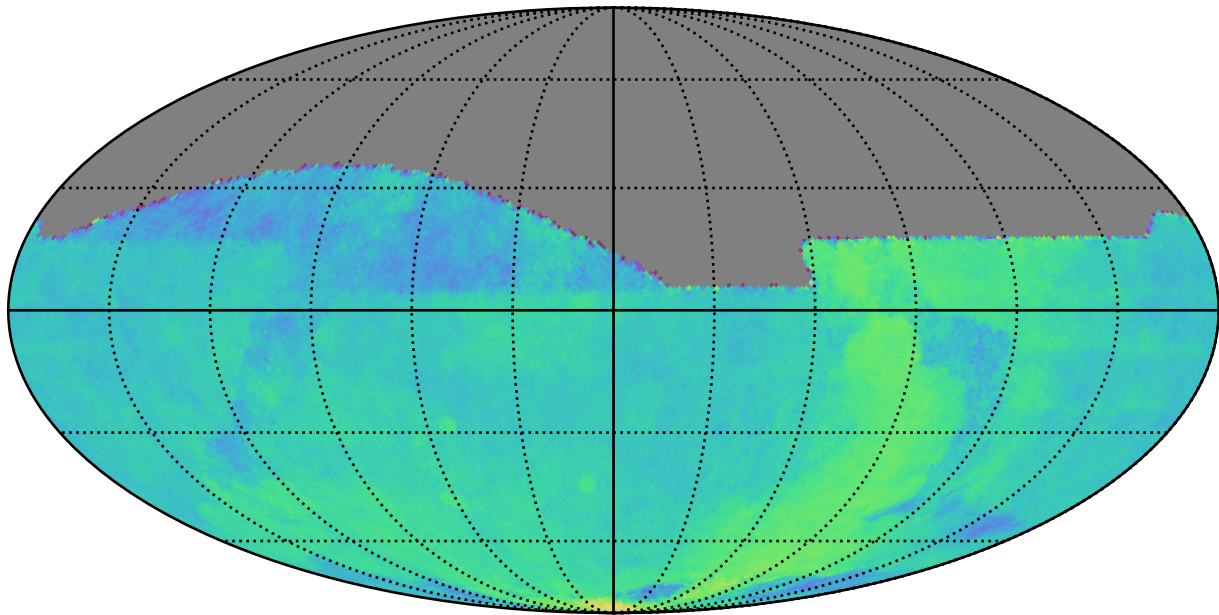
ddf_loaded_half_fl1_v3.4_10yrs All sky: Parallax Coverage @ 22.4
