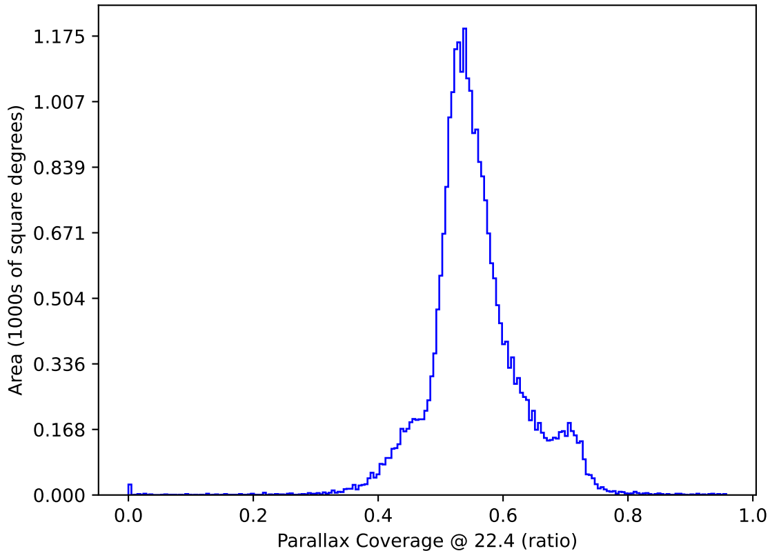
ddf_loaded_half_fl1_v3.4_10yrs All sky: Parallax Coverage @ 22.4
