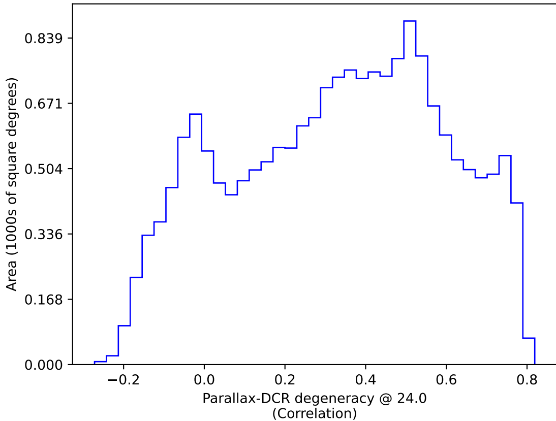
ddf_loaded_half_fl1_v3.4_10yrs WFD: Parallax-DCR degeneracy @ 24.0
