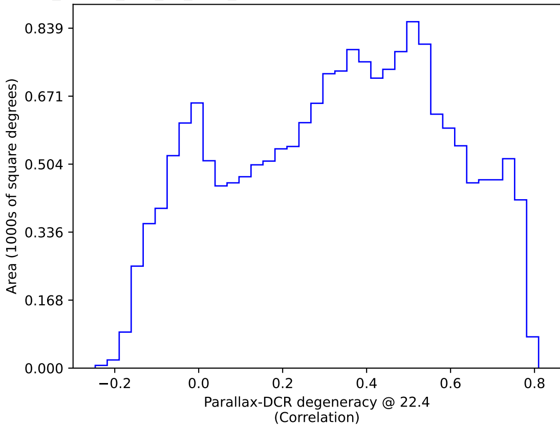
ddf_loaded_half_fl1_v3.4_10yrs WFD: Parallax-DCR degeneracy @ 22.4
