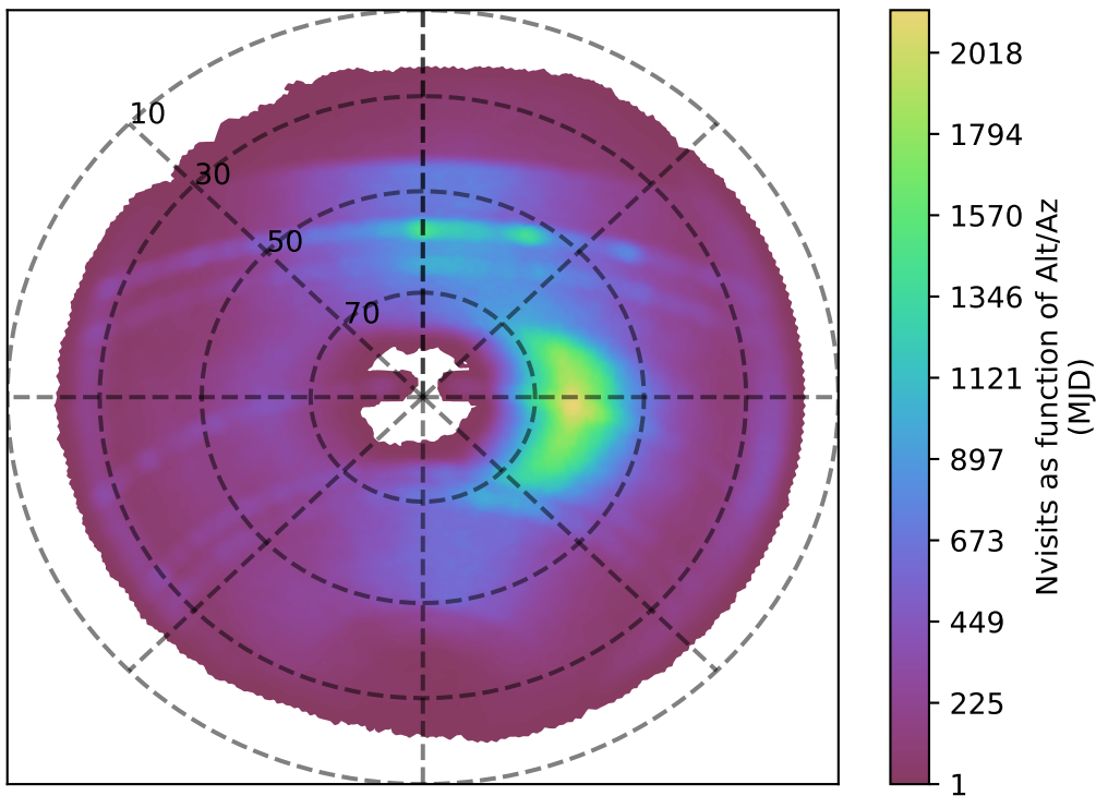
ddf_loaded_half_fl1_v3.4_10yrs z band: Nvisits as function of Alt/Az
