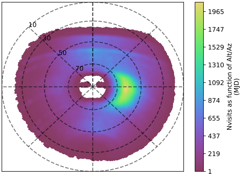
ddf_loaded_half_fl1_v3.4_10yrs y band: Nvisits as function of Alt/Az
