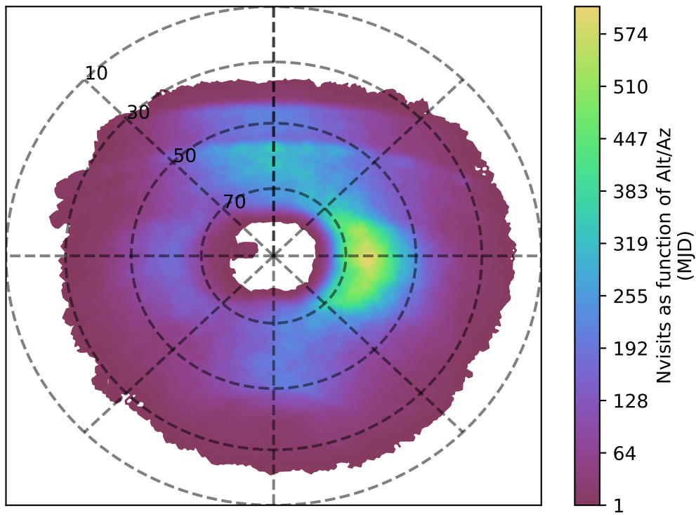
ddf_loaded_half_fl1_v3.4_10yrs u band: Nvisits as function of Alt/Az
