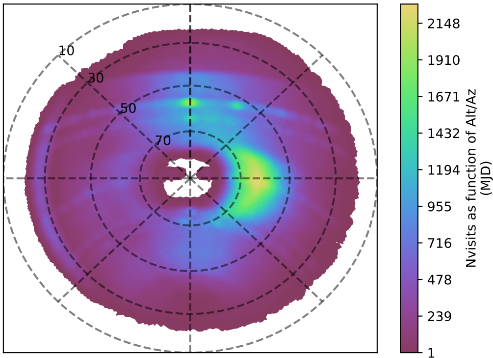
ddf_loaded_half_fl1_v3.4_10yrs r band: Nvisits as function of Alt/Az
