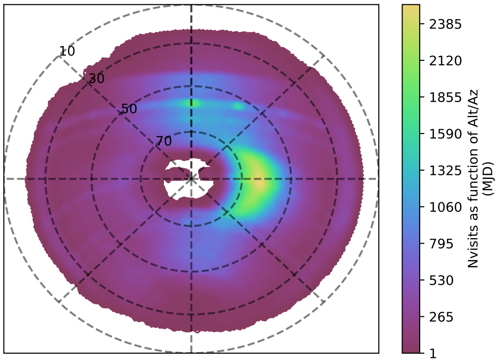
ddf_loaded_half_fl1_v3.4_10yrs i band: Nvisits as function of Alt/Az
