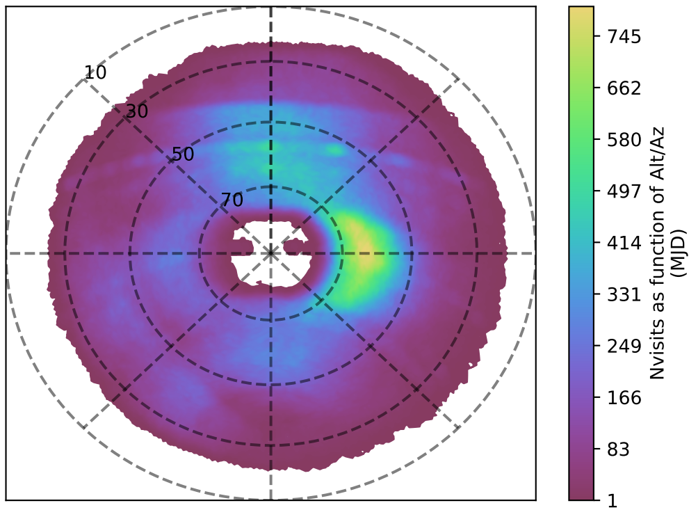
ddf_loaded_half_fl1_v3.4_10yrs g band: Nvisits as function of Alt/Az
