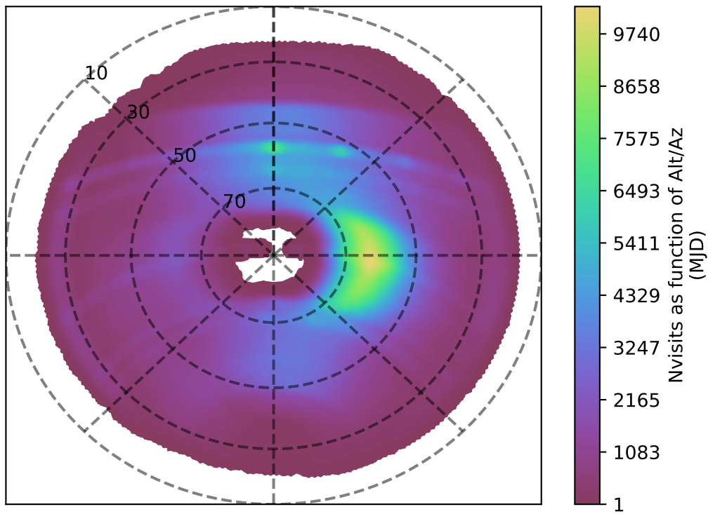
ddf_loaded_half_fl1_v3.4_10yrs all bands: Nvisits as function of Alt/Az
