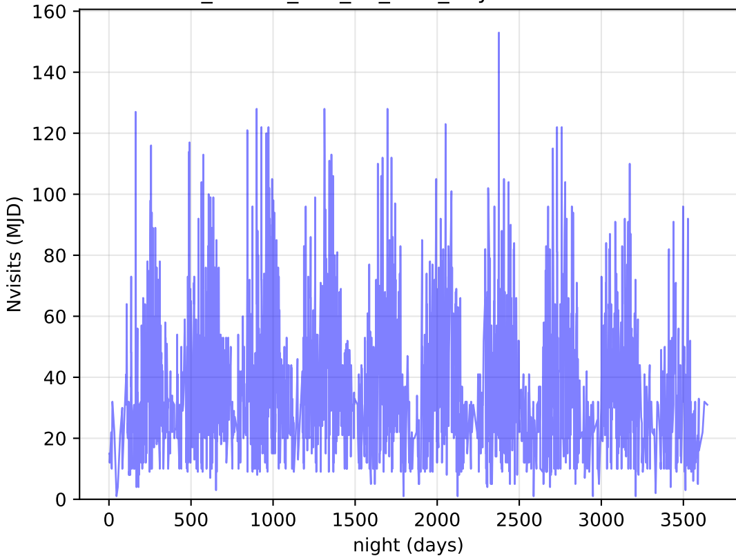
ddf_loaded_half_fl1_v3.4_10yrs DDF: Nvisits
