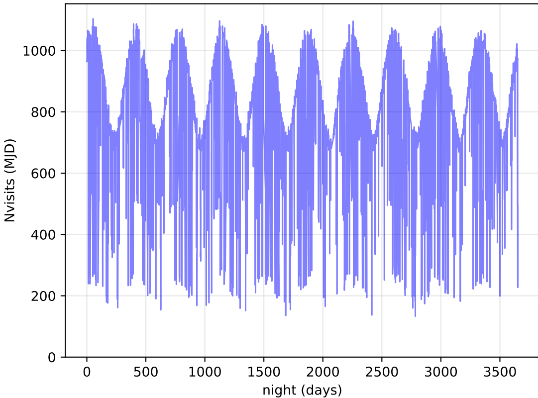
ddf_loaded_half_fl1_v3.4_10yrs All visits: Nvisits
