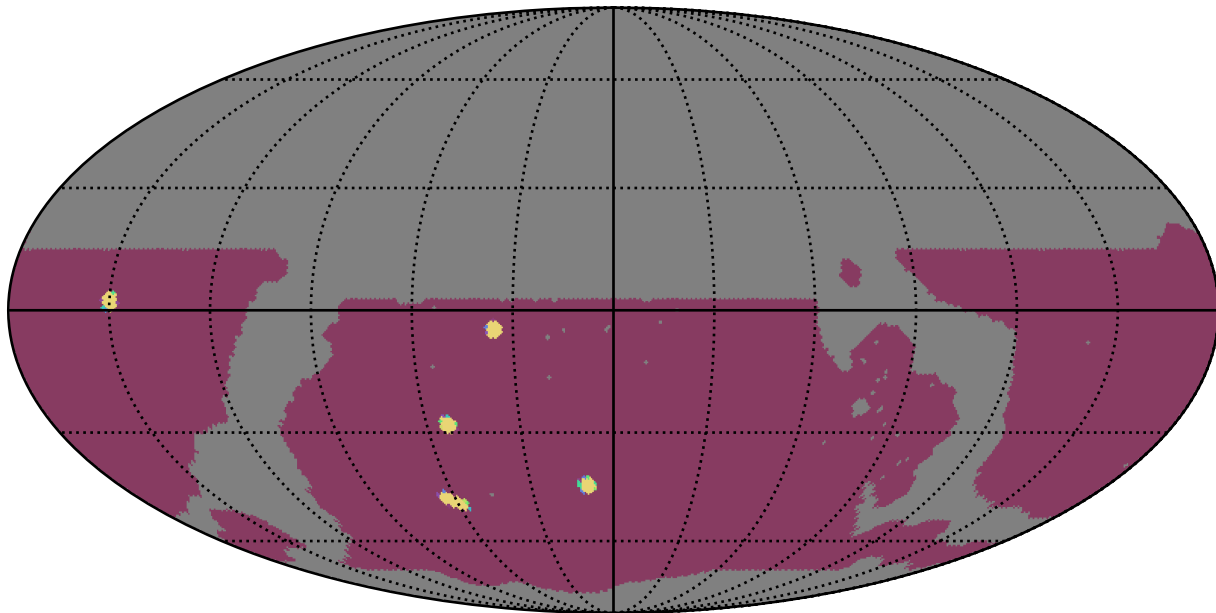
ddf_loaded_half_fl1_v3.4_10yrs WFD: NumberOfQuickRevisits
