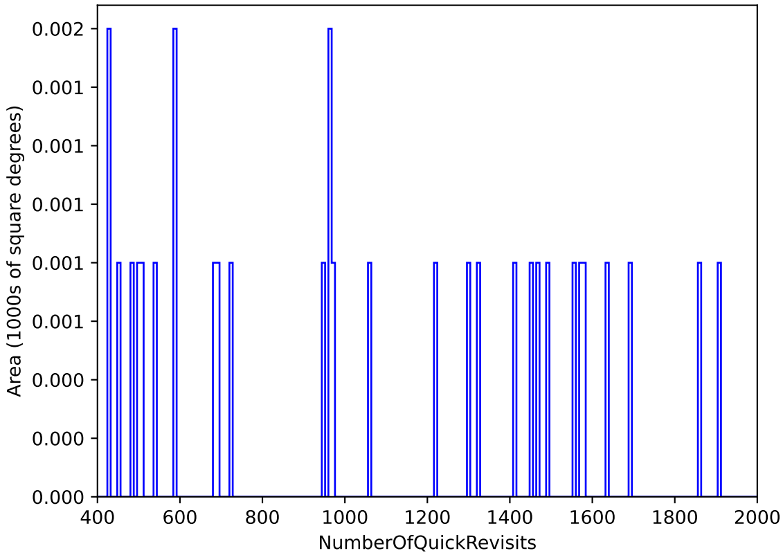
ddf_loaded_half_fl1_v3.4_10yrs WFD: NumberOfQuickRevisits
