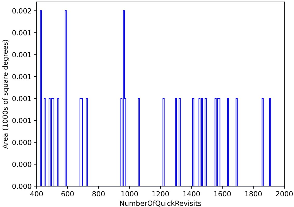
ddf_loaded_half_fl1_v3.4_10yrs All sky: NumberOfQuickRevisits
