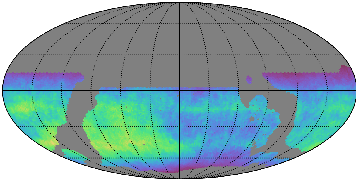
ddf_loaded_half_fl1_v3.4_10yrs WFD z band: Normalized Teff
