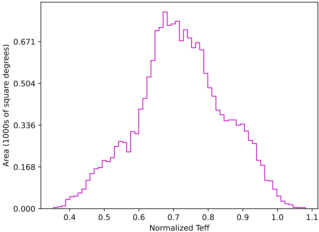
ddf_loaded_half_fl1_v3.4_10yrs WFD z band: Normalized Teff
