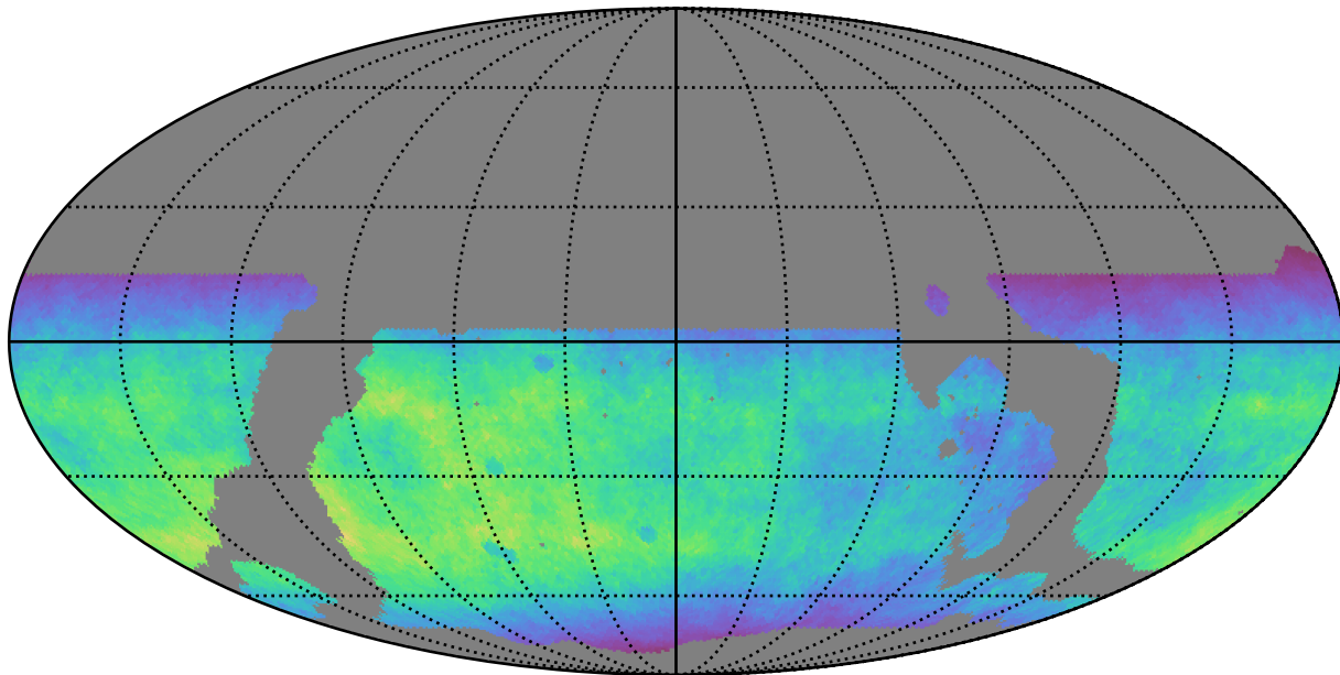
ddf_loaded_half_fl1_v3.4_10yrs WFD y band: Normalized Teff
