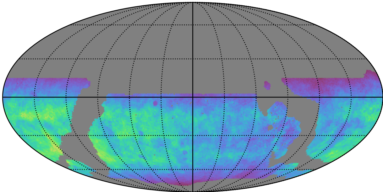
ddf_loaded_half_fl1_v3.4_10yrs WFD u band: Normalized Teff
