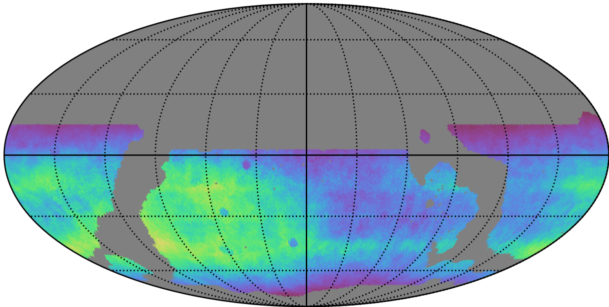
ddf_loaded_half_fl1_v3.4_10yrs WFD r band: Normalized Teff
