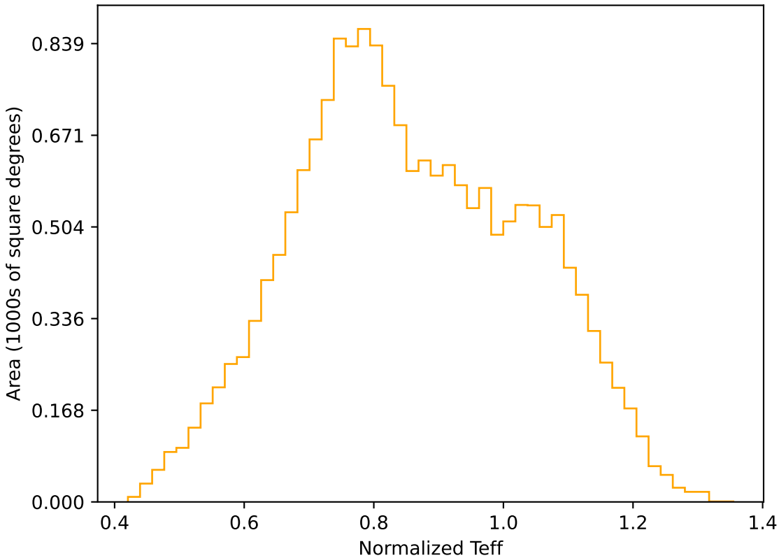
ddf_loaded_half_fl1_v3.4_10yrs WFD r band: Normalized Teff
