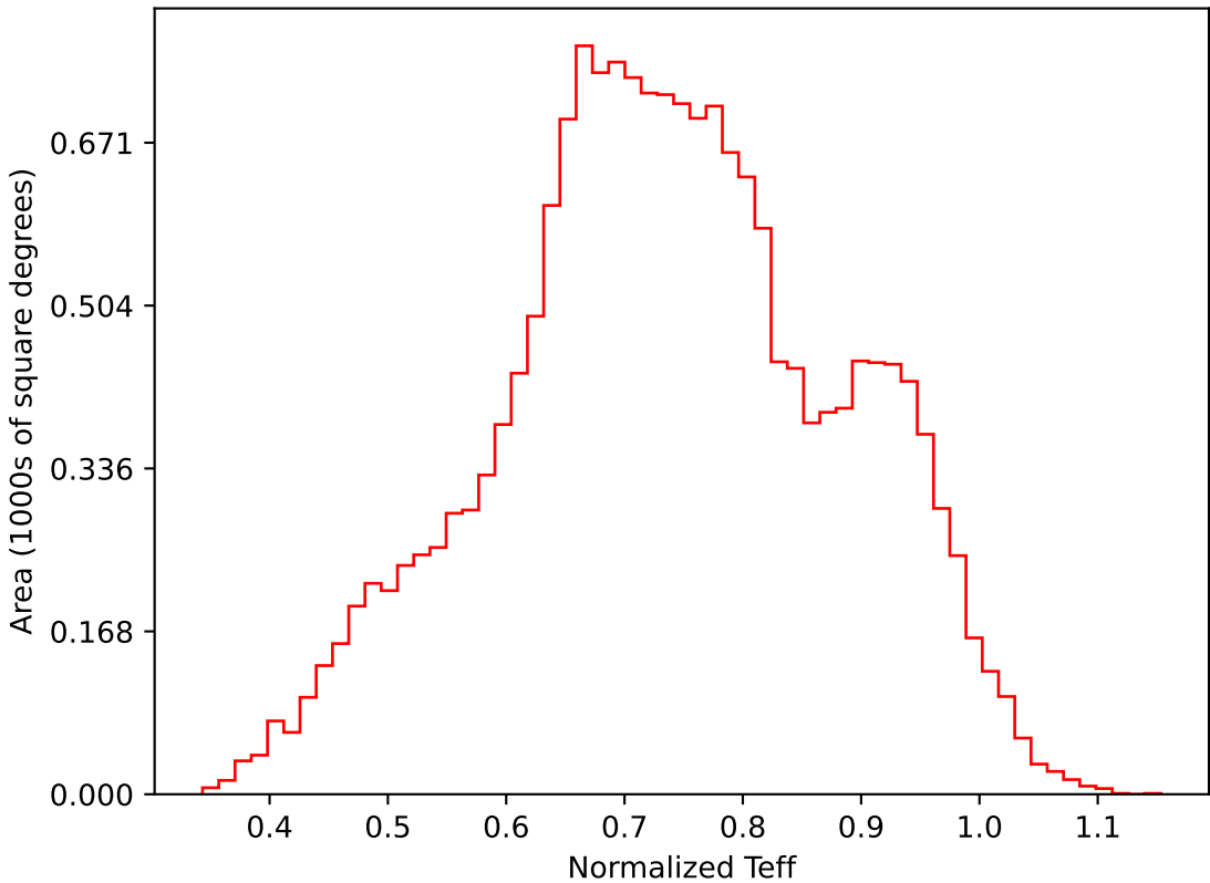
ddf_loaded_half_fl1_v3.4_10yrs WFD i band: Normalized Teff
