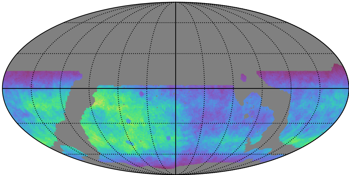
ddf_loaded_half_fl1_v3.4_10yrs WFD g band: Normalized Teff
