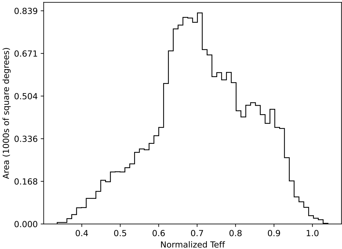
ddf_loaded_half_fl1_v3.4_10yrs WFD all bands: Normalized Teff
