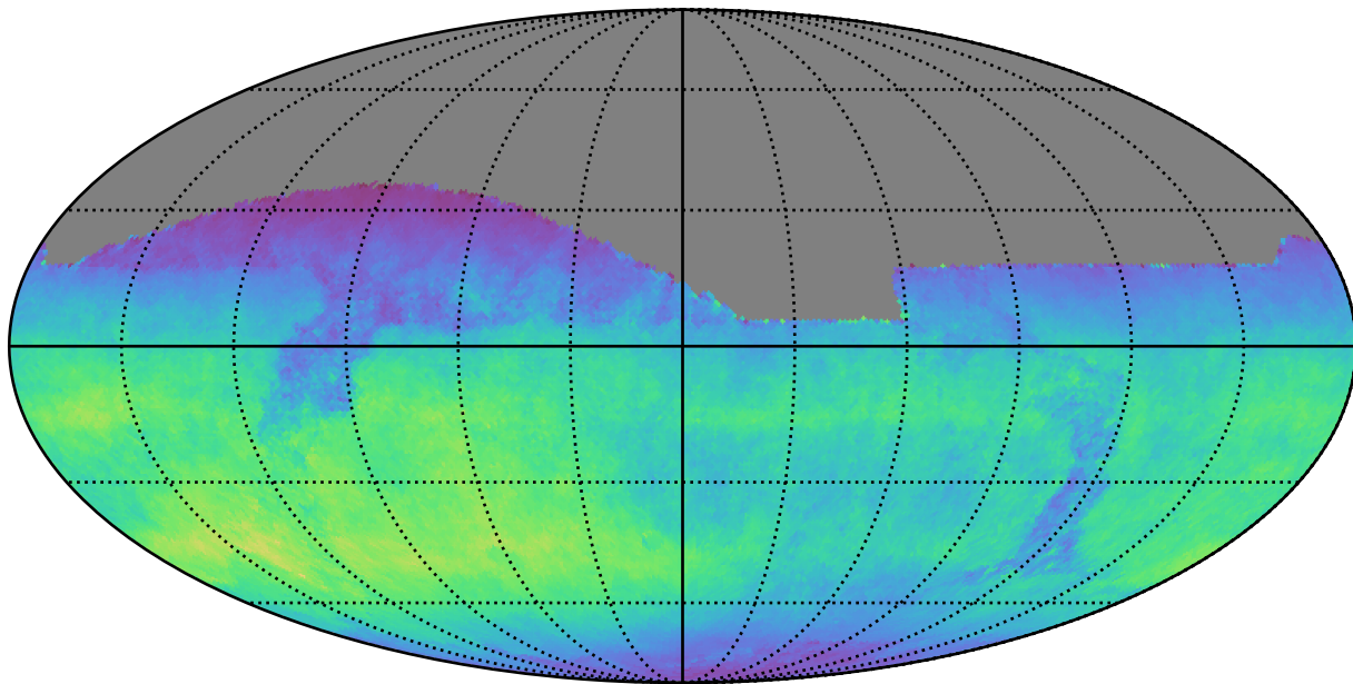
ddf_loaded_half_fl1_v3.4_10yrs All sky z band: Normalized Teff
