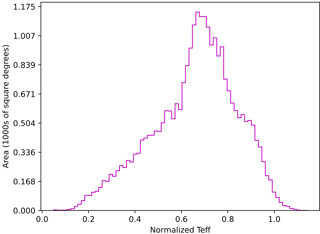
ddf_loaded_half_fl1_v3.4_10yrs All sky z band: Normalized Teff
