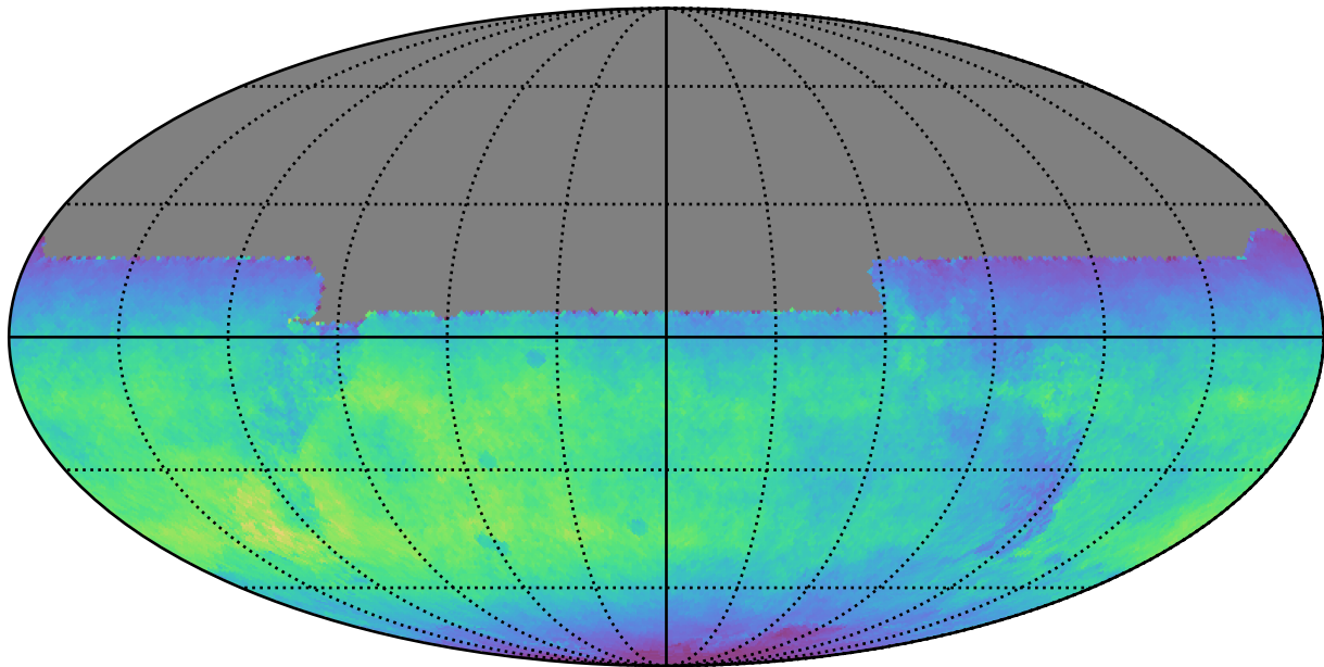
ddf_loaded_half_fl1_v3.4_10yrs All sky y band: Normalized Teff
