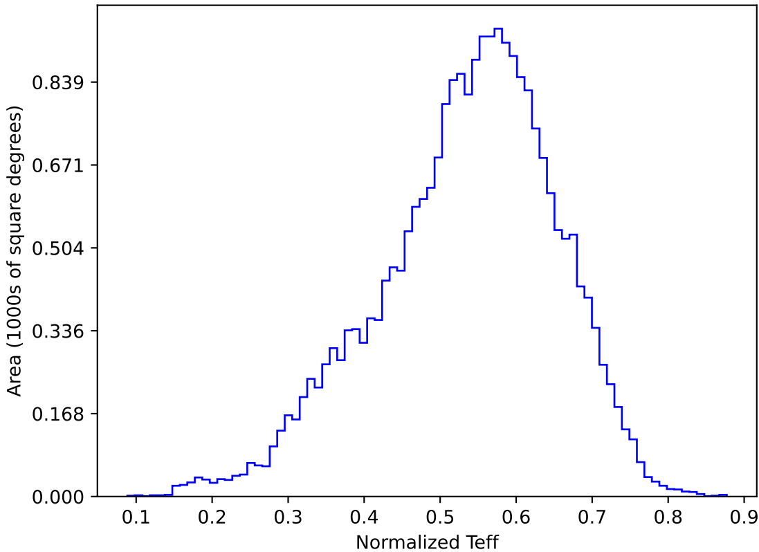
ddf_loaded_half_fl1_v3.4_10yrs All sky y band: Normalized Teff
