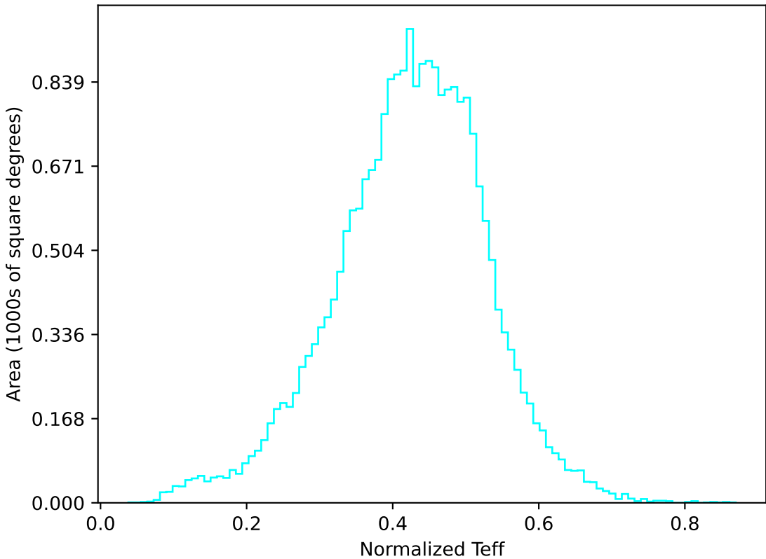
ddf_loaded_half_fl1_v3.4_10yrs All sky u band: Normalized Teff
