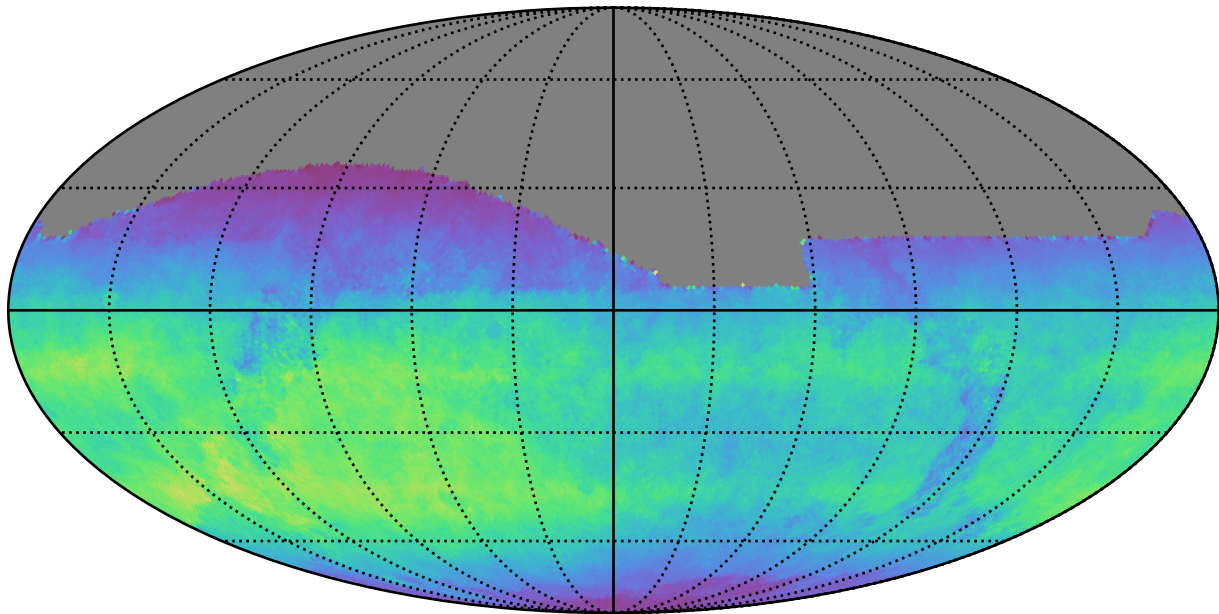
ddf_loaded_half_fl1_v3.4_10yrs All sky i band: Normalized Teff
