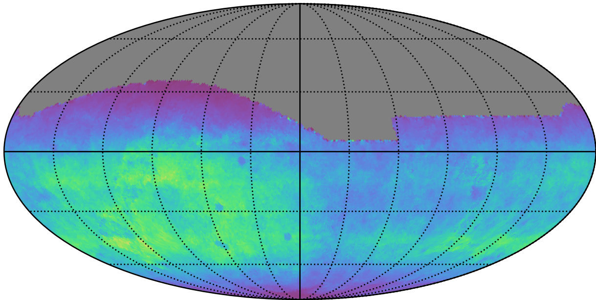
ddf_loaded_half_fl1_v3.4_10yrs All sky g band: Normalized Teff
