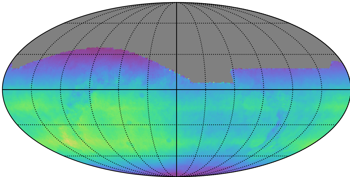
ddf_loaded_half_fl1_v3.4_10yrs All sky all bands: Normalized Teff
