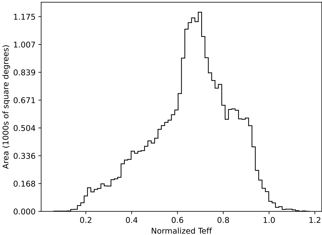
ddf_loaded_half_fl1_v3.4_10yrs All sky all bands: Normalized Teff
