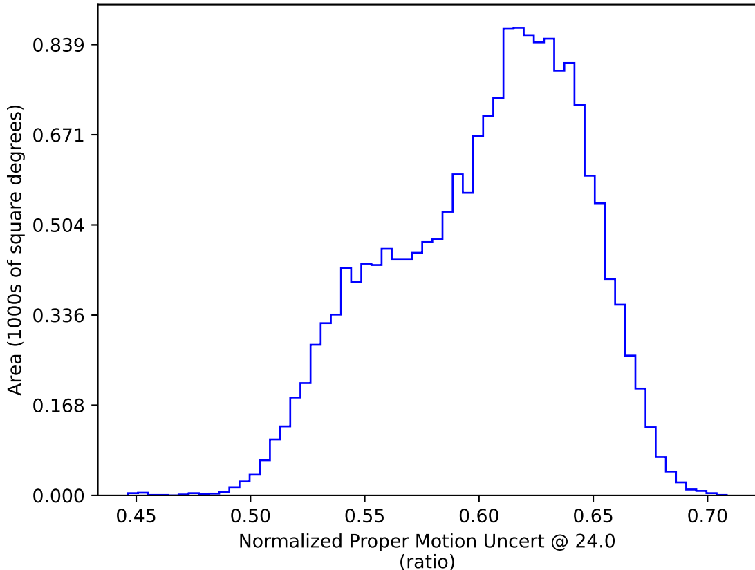
ddf_loaded_half_fl1_v3.4_10yrs WFD: Normalized Proper Motion Uncert @ 24.0
