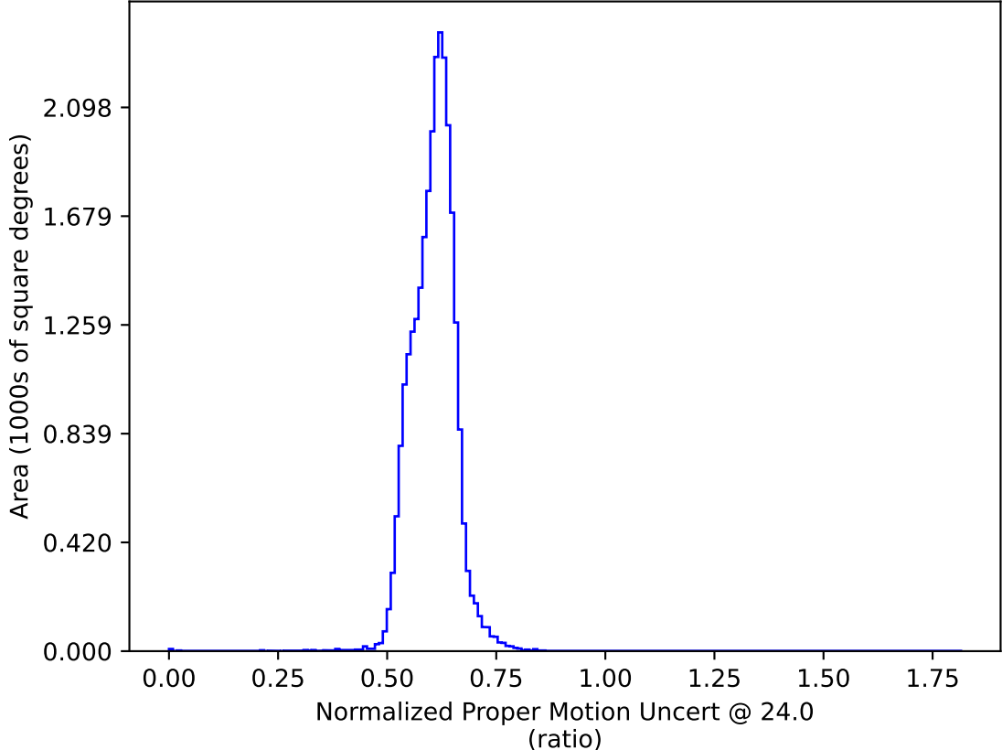
ddf_loaded_half_fl1_v3.4_10yrs All sky: Normalized Proper Motion Uncert @ 24.0
