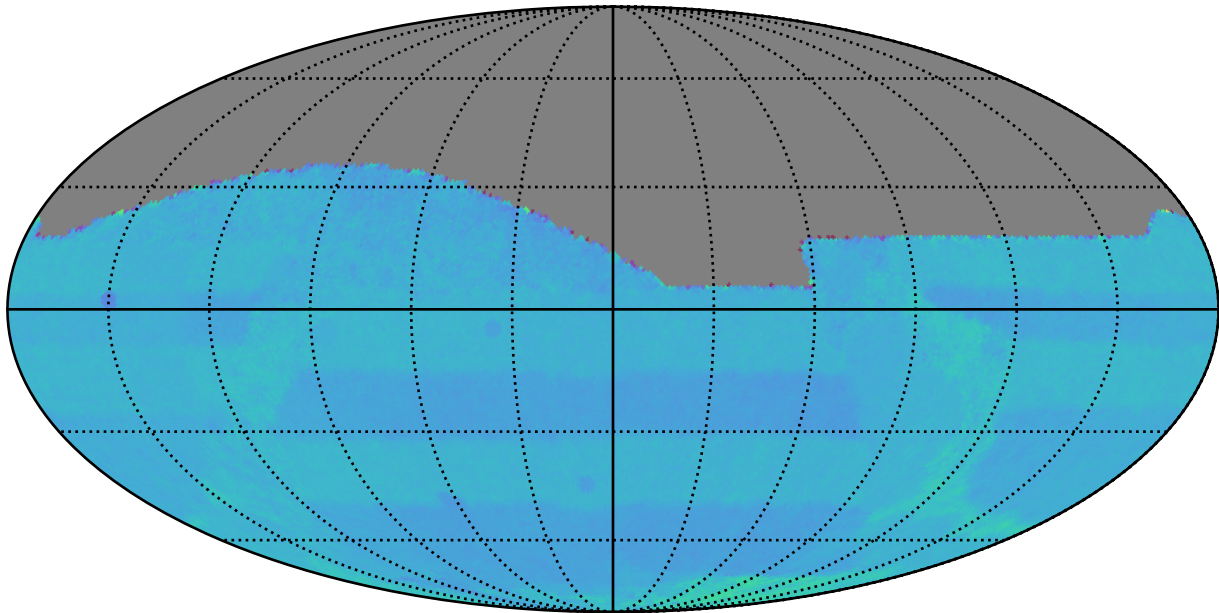
ddf_loaded_half_fl1_v3.4_10yrs All sky: Normalized Proper Motion Uncert @ 20.5
