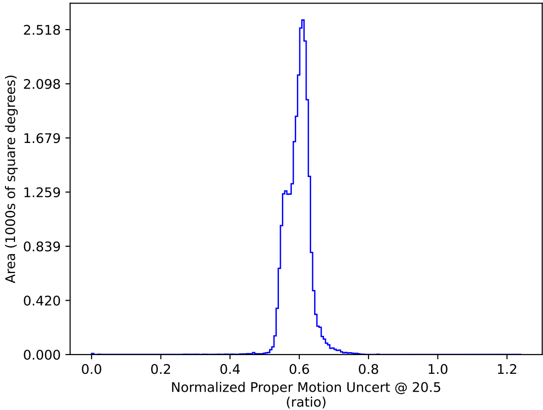
ddf_loaded_half_fl1_v3.4_10yrs All sky: Normalized Proper Motion Uncert @ 20.5
