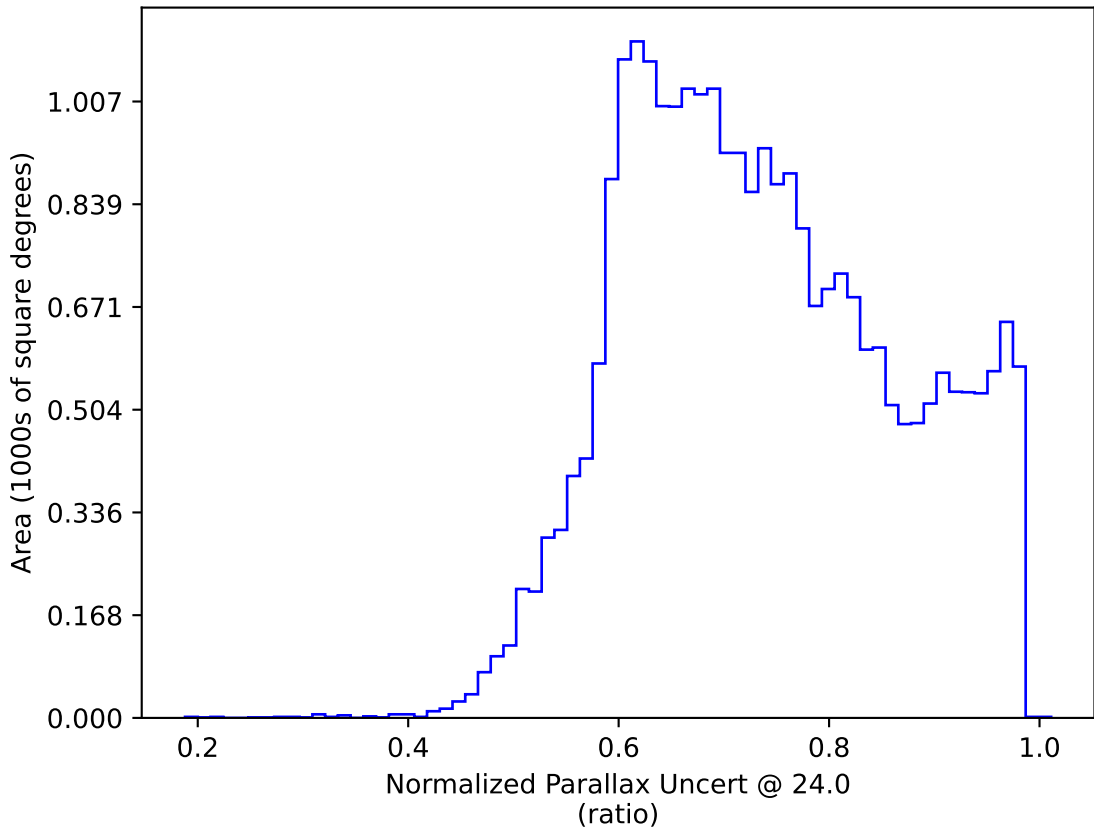
ddf_loaded_half_fl1_v3.4_10yrs All sky: Normalized Parallax Uncert @ 24.0
