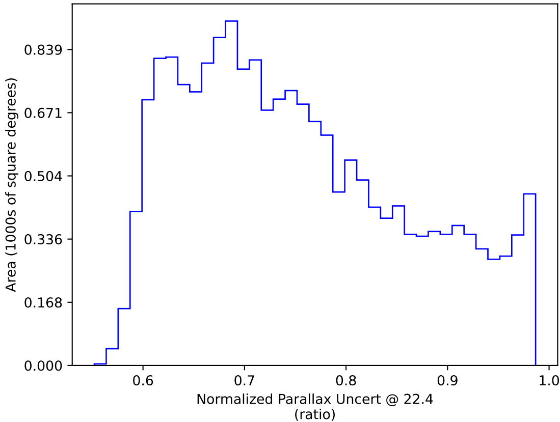
ddf_loaded_half_fl1_v3.4_10yrs WFD: Normalized Parallax Uncert @ 22.4
