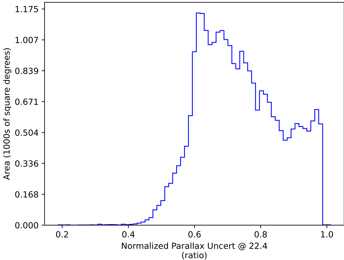
ddf_loaded_half_fl1_v3.4_10yrs All sky: Normalized Parallax Uncert @ 22.4
