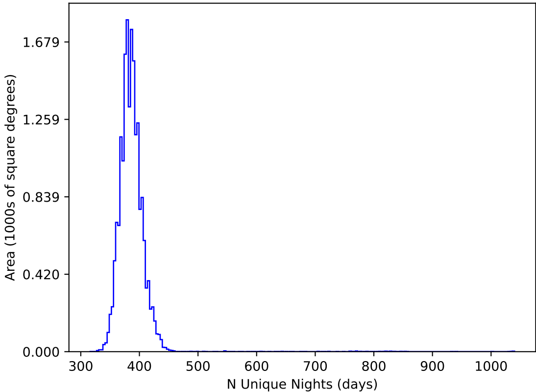
ddf_loaded_half_fl1_v3.4_10yrs WFD all bands: N Unique Nights
