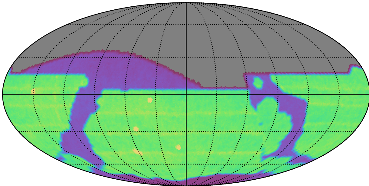
ddf_loaded_half_fl1_v3.4_10yrs All sky all bands: N Unique Nights
