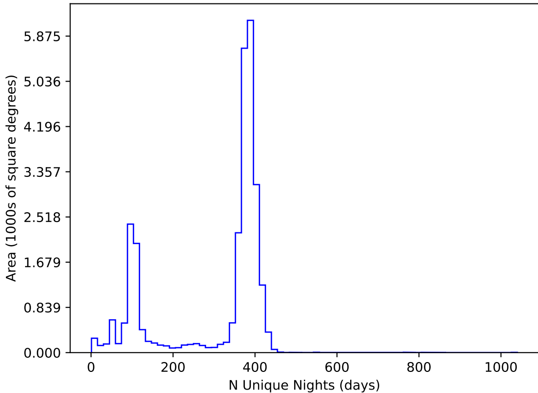
ddf_loaded_half_fl1_v3.4_10yrs All sky all bands: N Unique Nights
