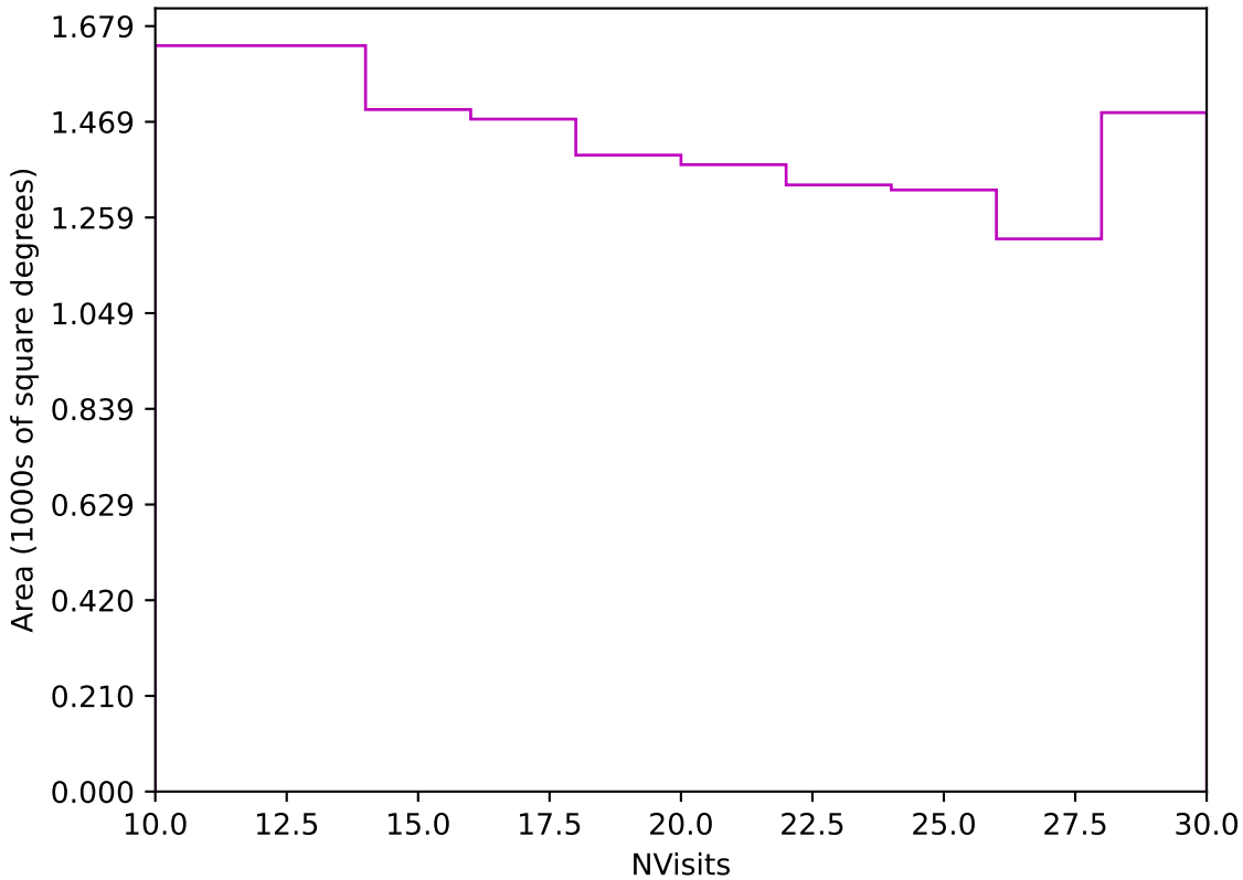
ddf_loaded_half_fl1_v3.4_10yrs Yr 3-4 z band: NVisits
