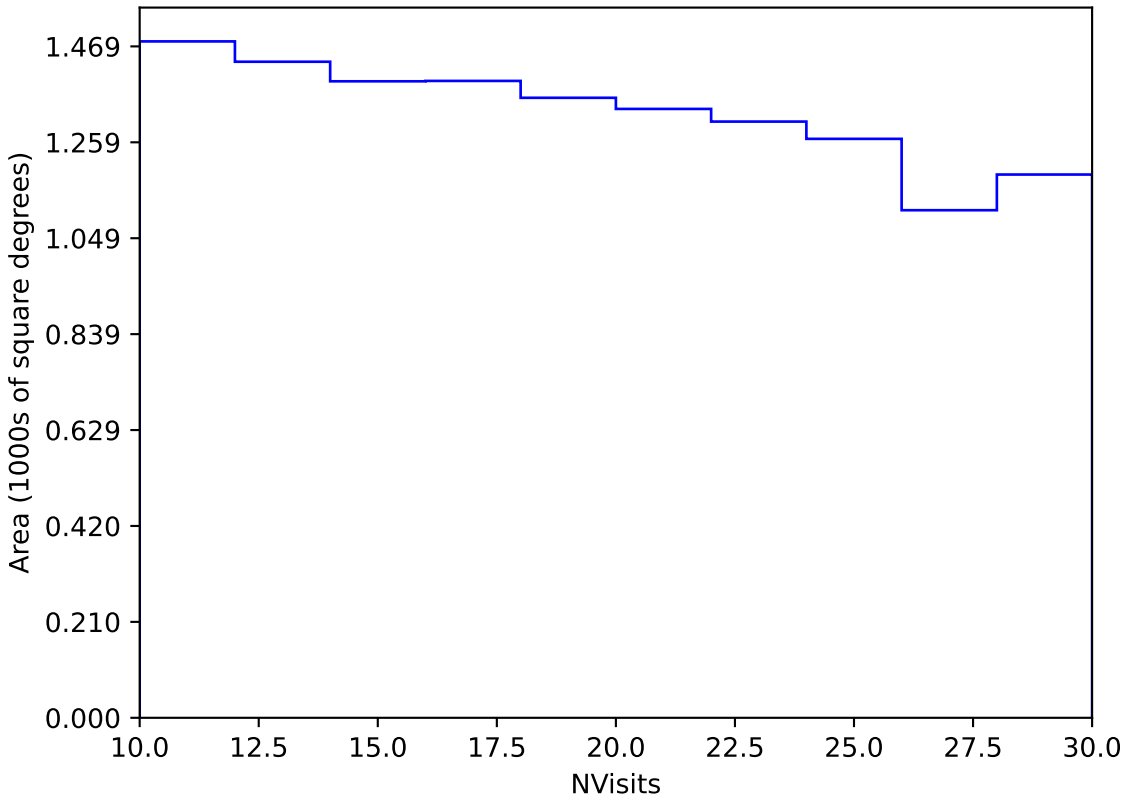
ddf_loaded_half_fl1_v3.4_10yrs Yr 3-4 y band: NVisits
