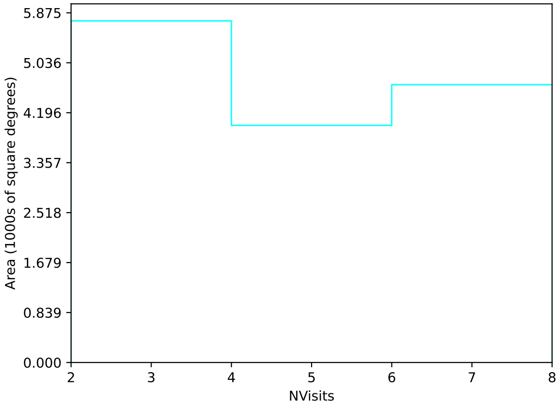
ddf_loaded_half_fl1_v3.4_10yrs Yr 3-4 u band: NVisits
